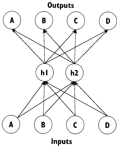
FIG. 1. Feedforward network. Input units are drawn at the bottom; output units are drawn at the top. Connections between nodes are drawn as arrows.
