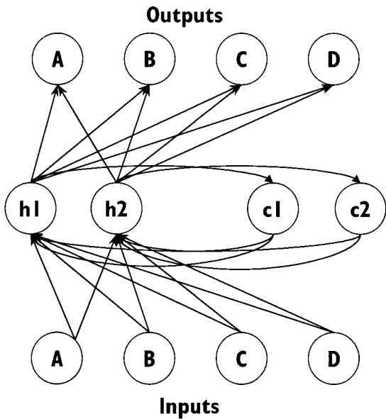
FIG. 2. Simple recurrent network. The context layer consists of the units marked c1 and c2 . Connections from h1 to c1 and from h2 to c2 are fixed at 1.0; all other weights are modifiable. See text for further details.
